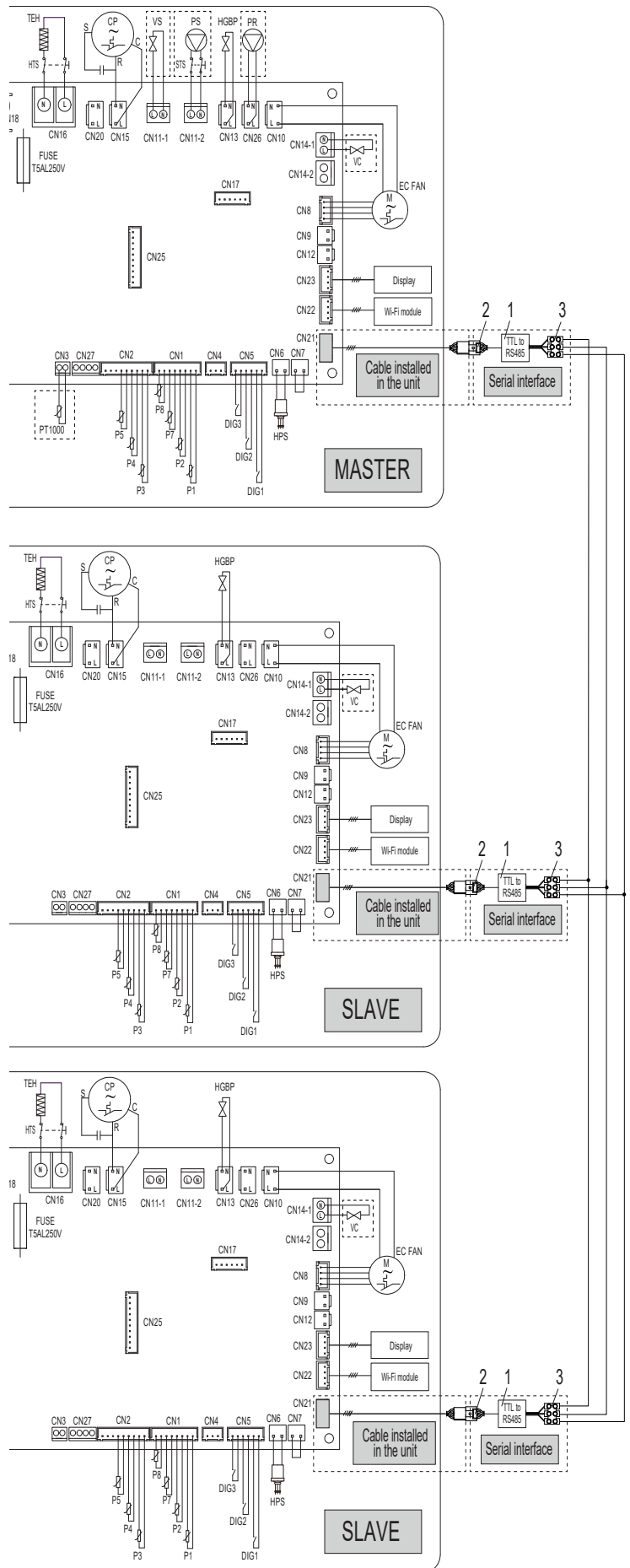
fig. 72 - Cascade wiring diagram
