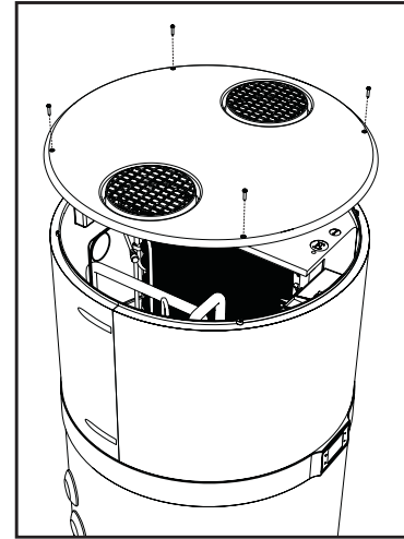
fig. 74- Top cover removal
