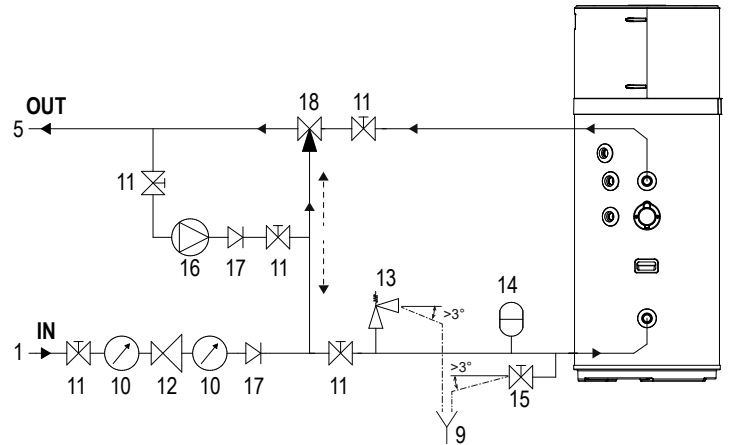
fig. 60 - Example of water system WITH thermostatic mixing valve (recirculation on unit cold water inlet connection)
