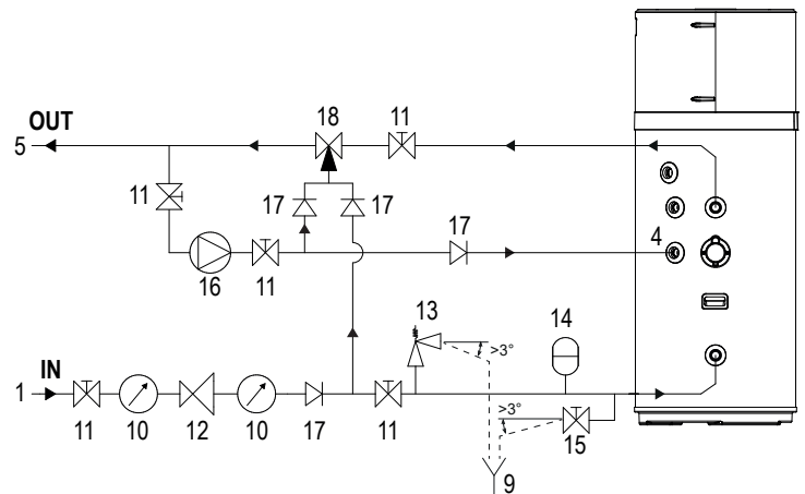
fig. 61 - Example of water system WITH thermostatic mixing valve (recirculation on unit water recirculation connection)
